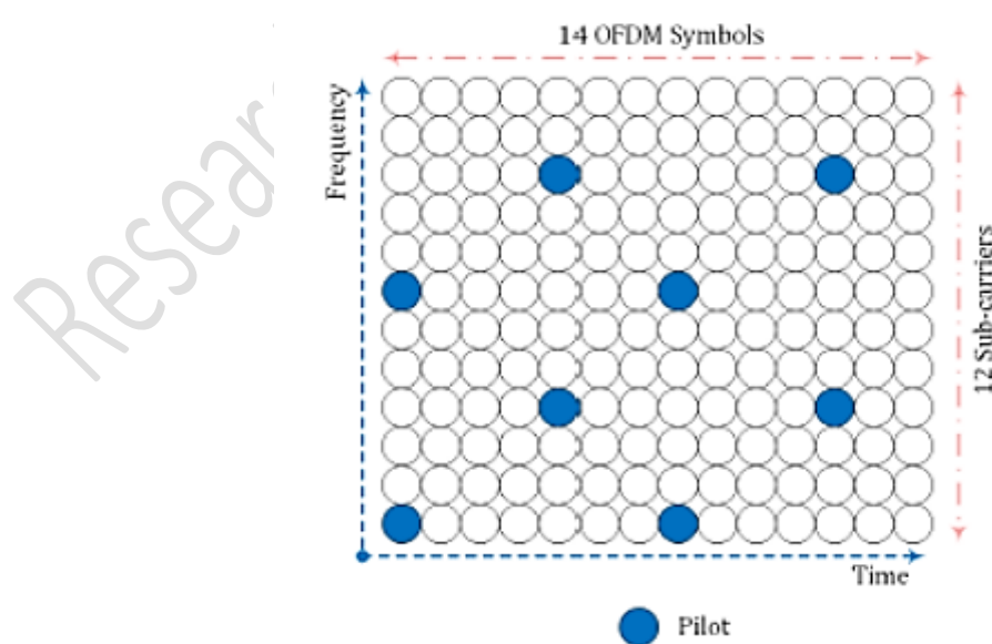
Figure 1:- An example of the time-frequency resource grid for LTE-A
