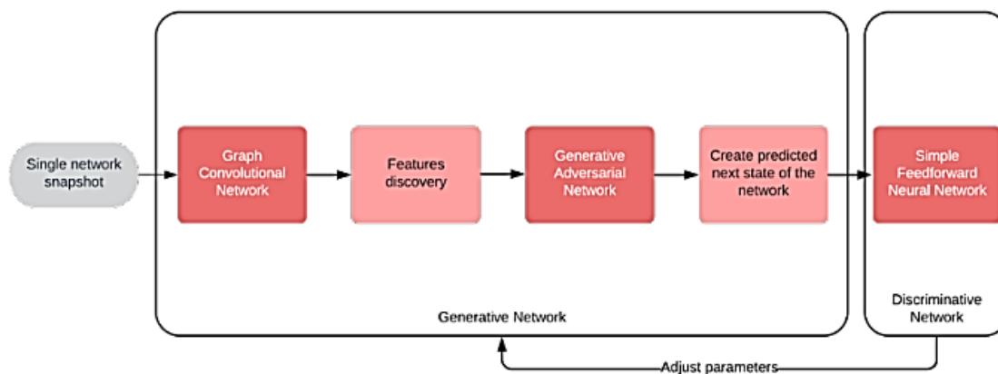
Figure 1: GCN-GAN flowchart
