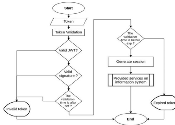
JWT Authentication flow diagram
